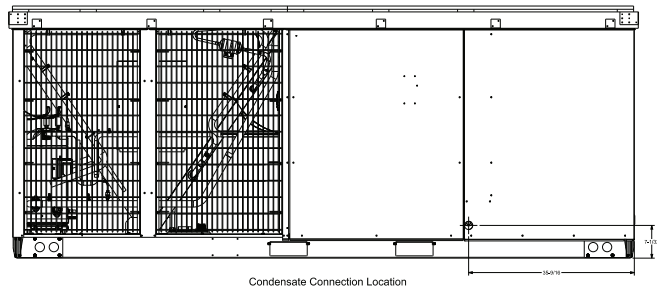
Condensate Connection Location
